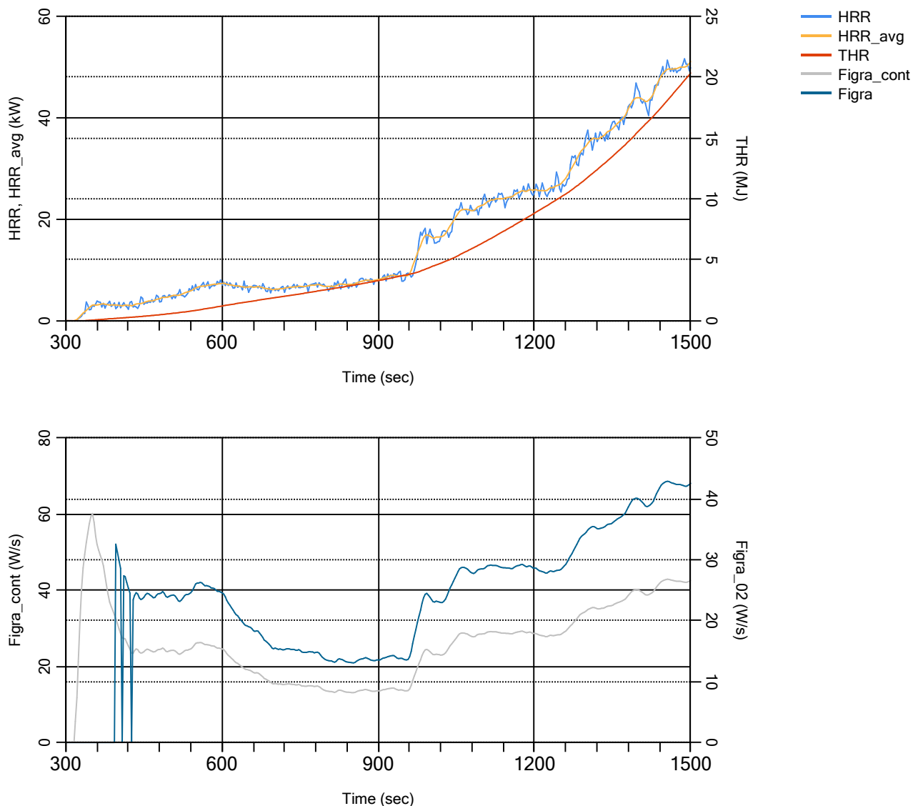
Heat release and Figra
